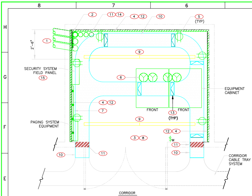
TYPICAL ENTRANCE TELECOMMUNICATIONS ROOM SCALE: NONE
