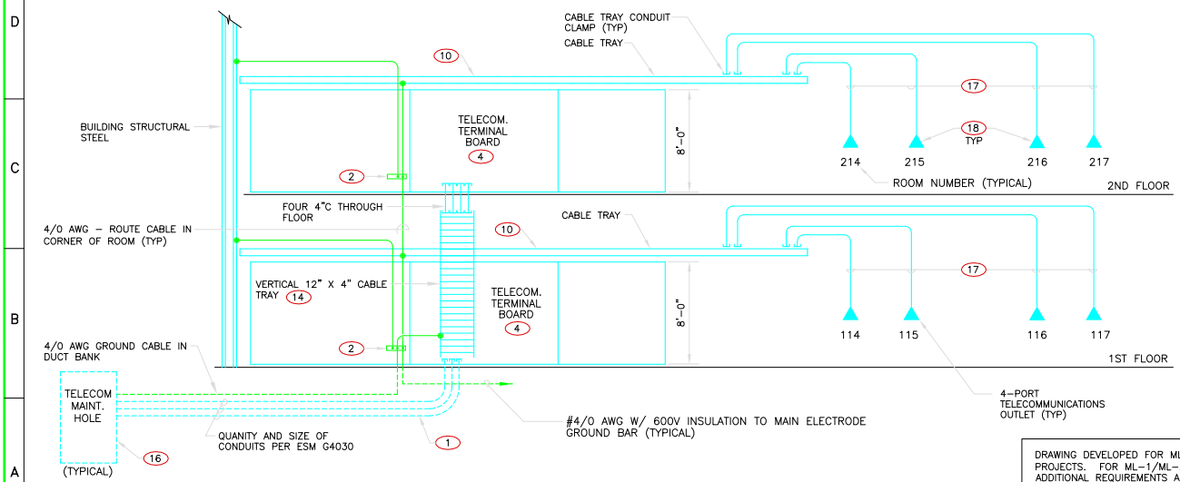
TELECOMMUNICATIONS RISER DIAGRAM SCALE: NONE
