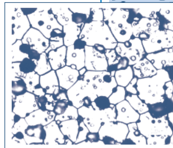
Figure 3: Optical micrographs of surrogate fuel pellets sintered at 1400\ ^\circ C and 1700\ ^\circ C .
