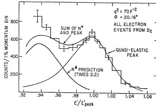
FIG. 20. Total scattered electron spectrum from deuterium target, q^2 = 70 F^{-2} .
