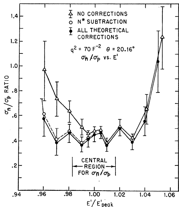
FIG. 32. (\sigma_n/\sigma_p) ratios versus E' at q^2=70 F^{-2} .
