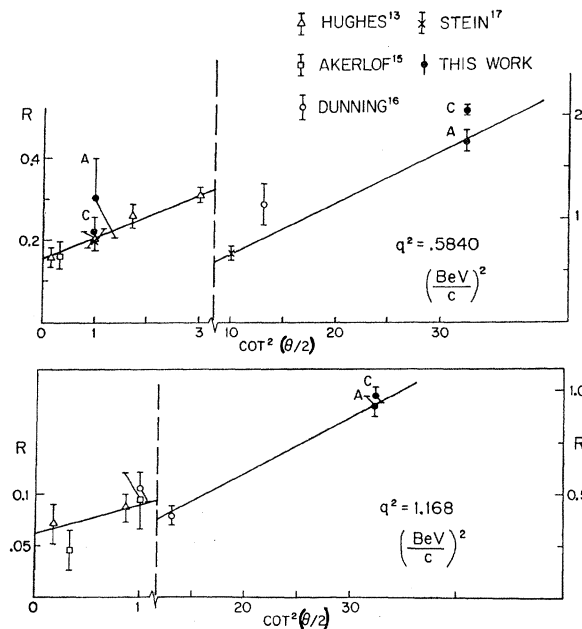
FIG. 43. Plots of R = \sigma_{\text{neutron}} / [\sigma_{\text{Mott}} \times (E/E') \times \tan^2(\frac{1}{2}\theta) \times (1+\tau)^{-1}] for q^2 = 0.5840 and 1.168 (\text{BeV}/c)^2 to show method of extracting form factors. C = coincidence method data; A = area-method data.
