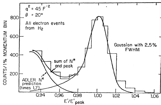
FIG. 15. Scattered electron spectrum at q^2 = 45 \text{ F}^{-2} , from hydrogen target.
