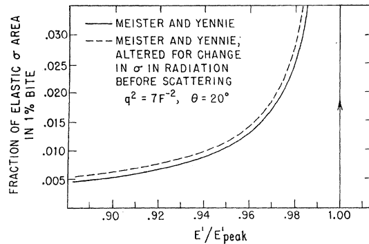
FIG. 12. Hydrogen radiative tails at q^2 = 7 \text{ F}^{-2} .
