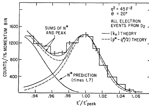
FIG. 19. Total scattered electron spectrum from D_2 target, q^2 = 45 F^{-2} .
