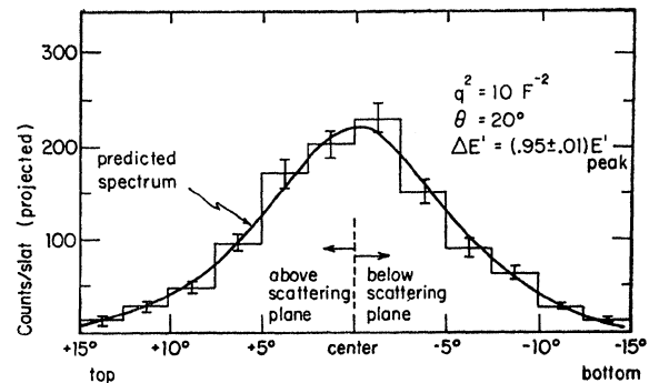
FIG. 39. Proton angular distribution projected sideways, q^2 = 10 \text{ F}^{-2} for electrons below the peak position.
