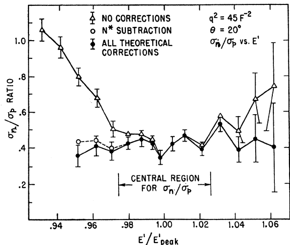
FIG. 31. (\sigma_n/\sigma_p) ratios versus E' at q^2=45 F^{-2} .
