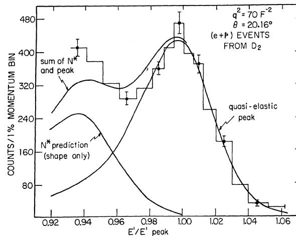
FIG. 17. Scattered electron spectrum with coincident proton from D 2 target, q^2 = 70 \text{ F}^{-2} .
