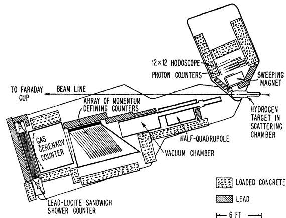
FIG. 1. Schematic plan—view of the apparatus.
