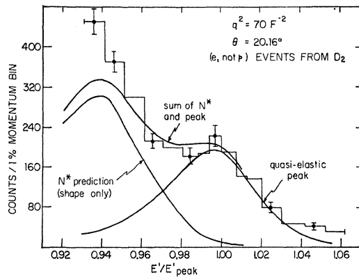
FIG. 18. Scattered electron spectrum without coincident proton from D_2 target, q^2 = 70 F^{-2} .
